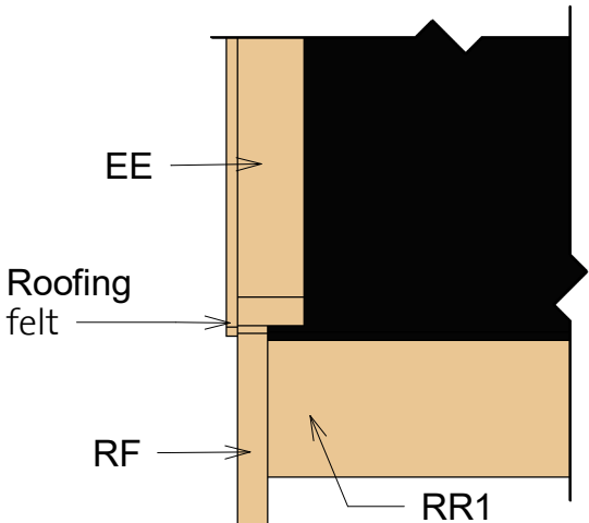
3) Roof Reinforcement
